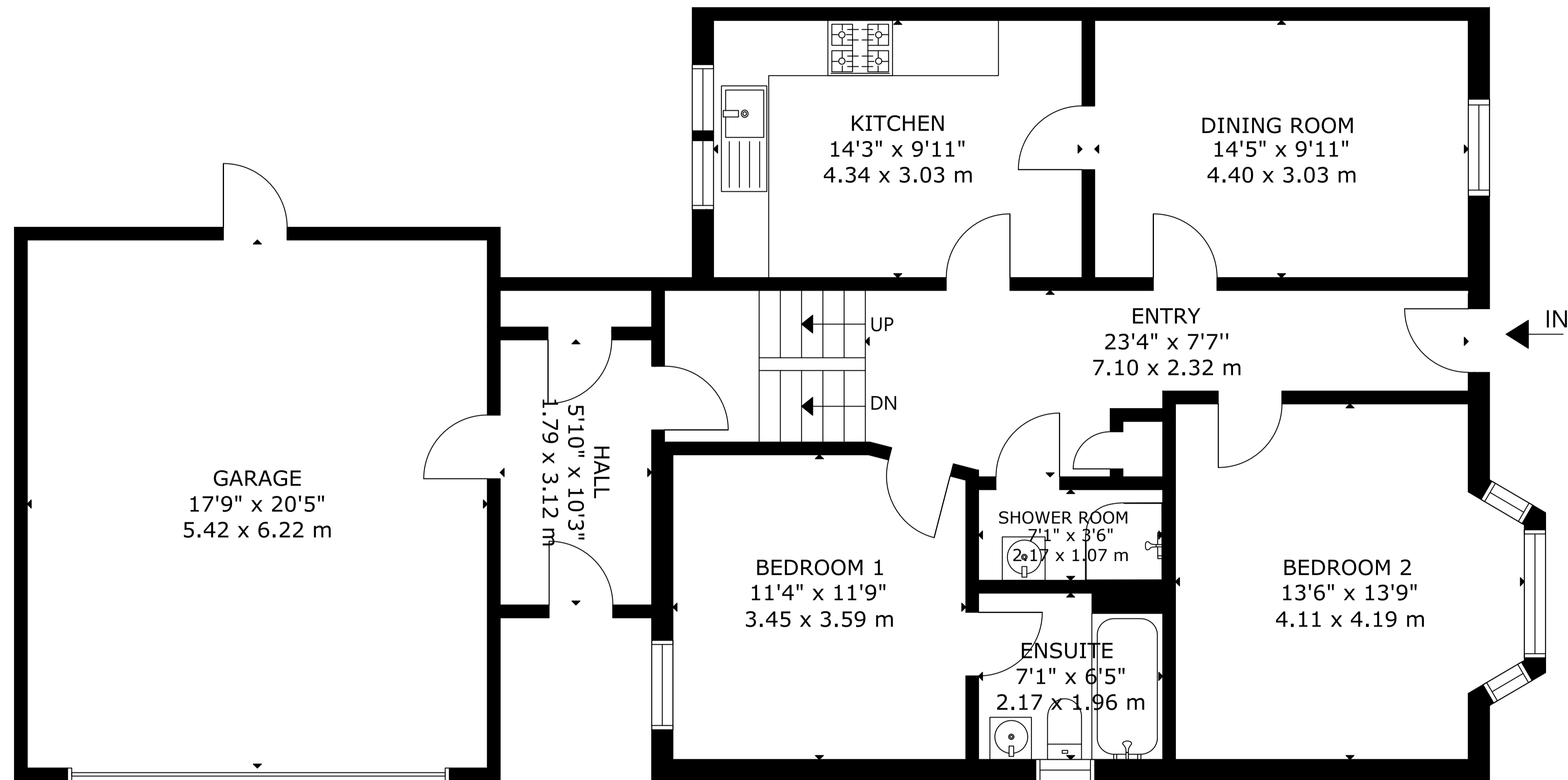
GROUND FLOOR
