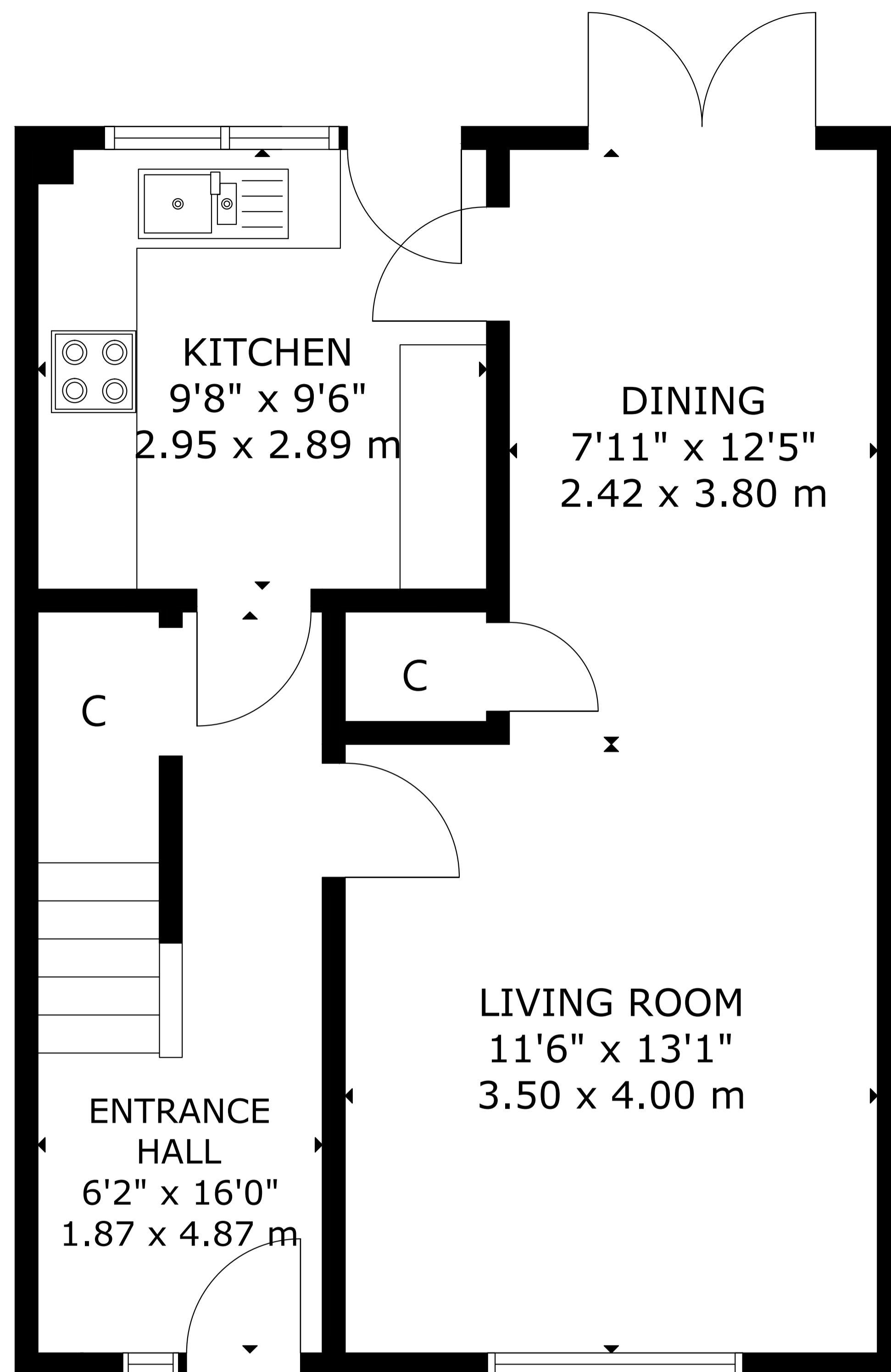
GROUND FLOOR
