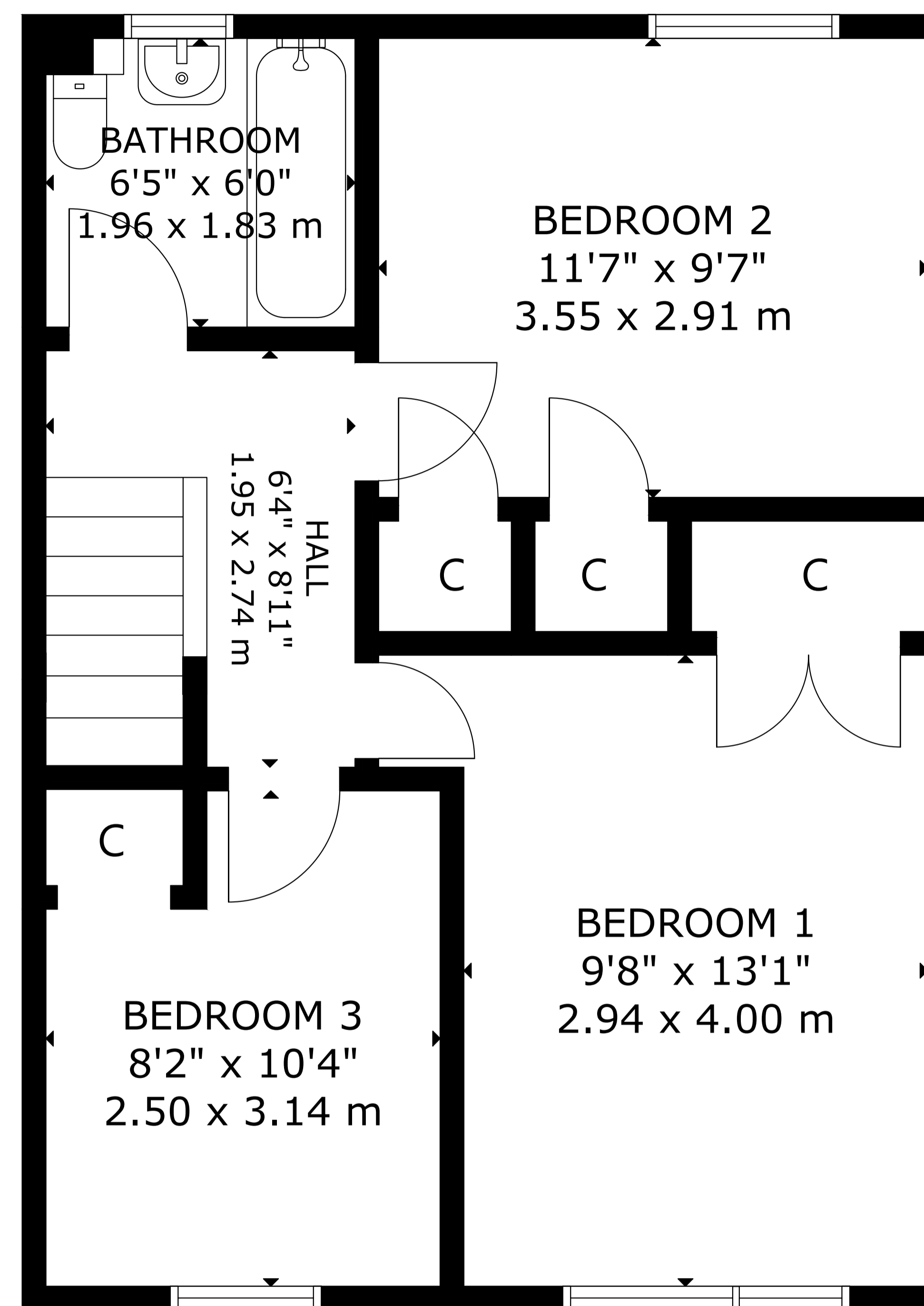
FIRST FLOOR
